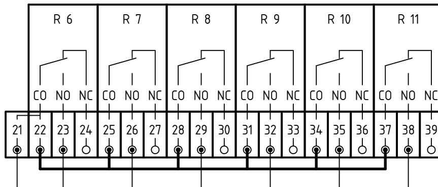
Expansion board (R8-6, R8-11 models only)
