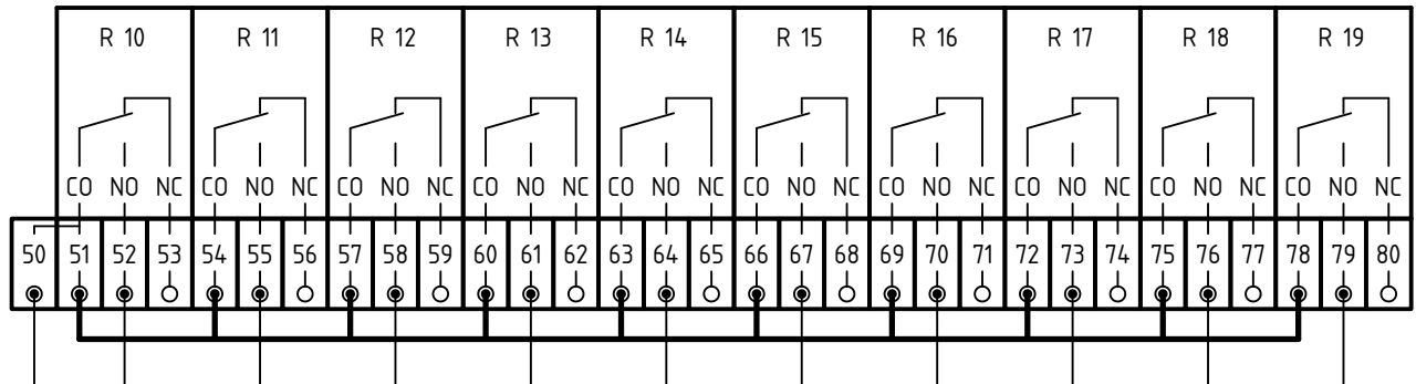
Extension board (R4-6 only)
